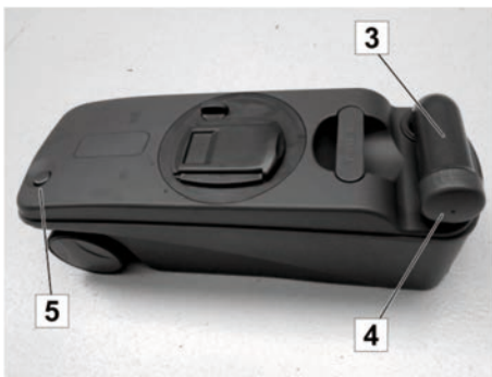
Fig. 193: Emptying the waste holding tank
